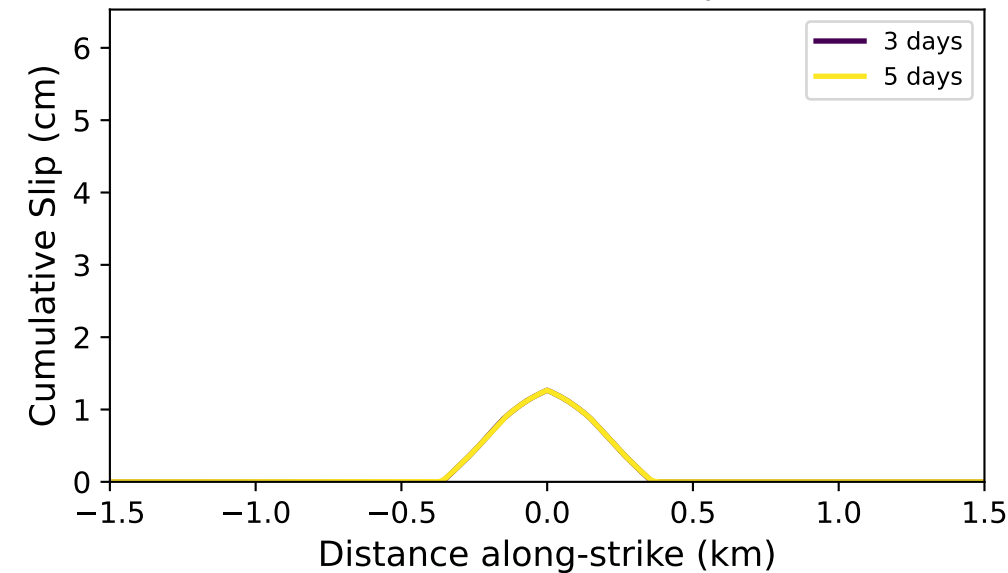
Job 632881: \tau_0 = 15.00 MPa, k_{pmax} fixed perm
