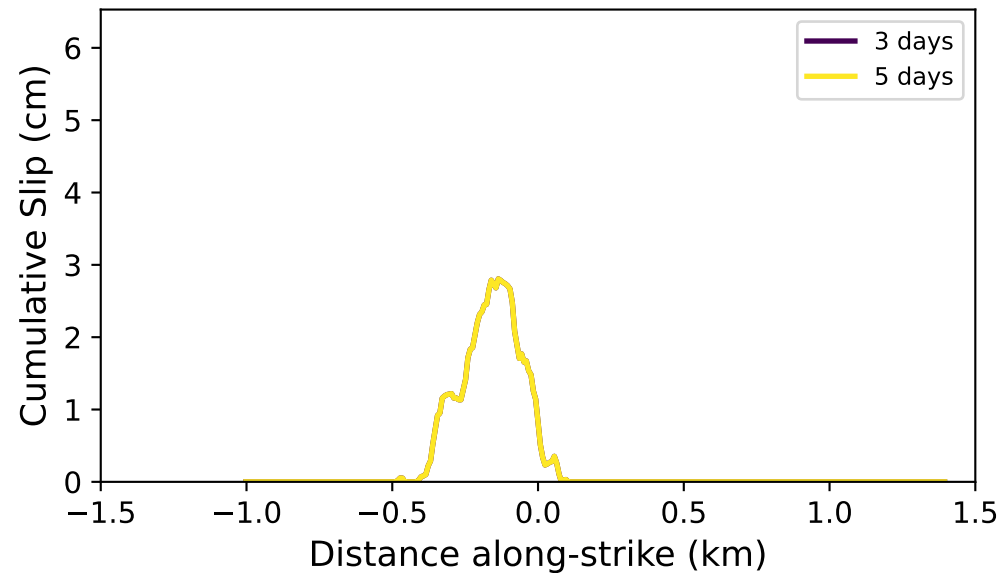
Job 632875: \tau_0 = 10.36 MPa, k_{pmax} 2.5e-13
