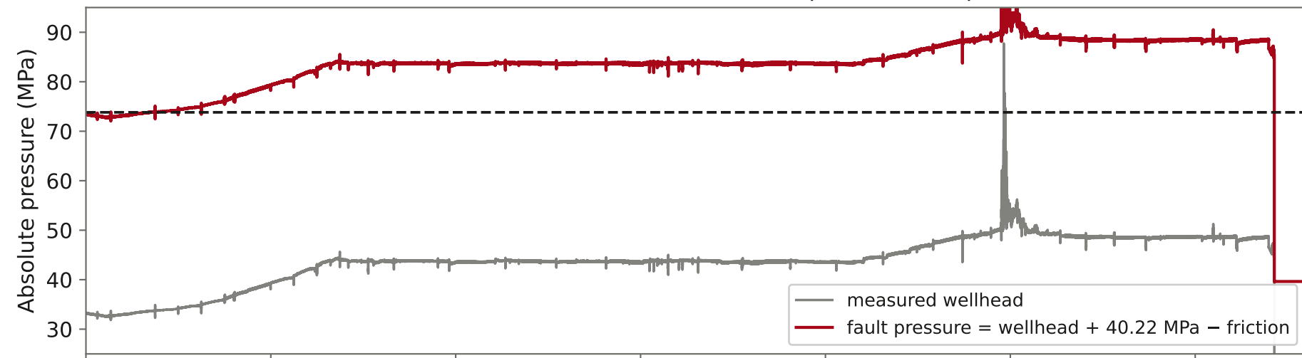
(a) Measured wellhead, and the fault pressure it implies
