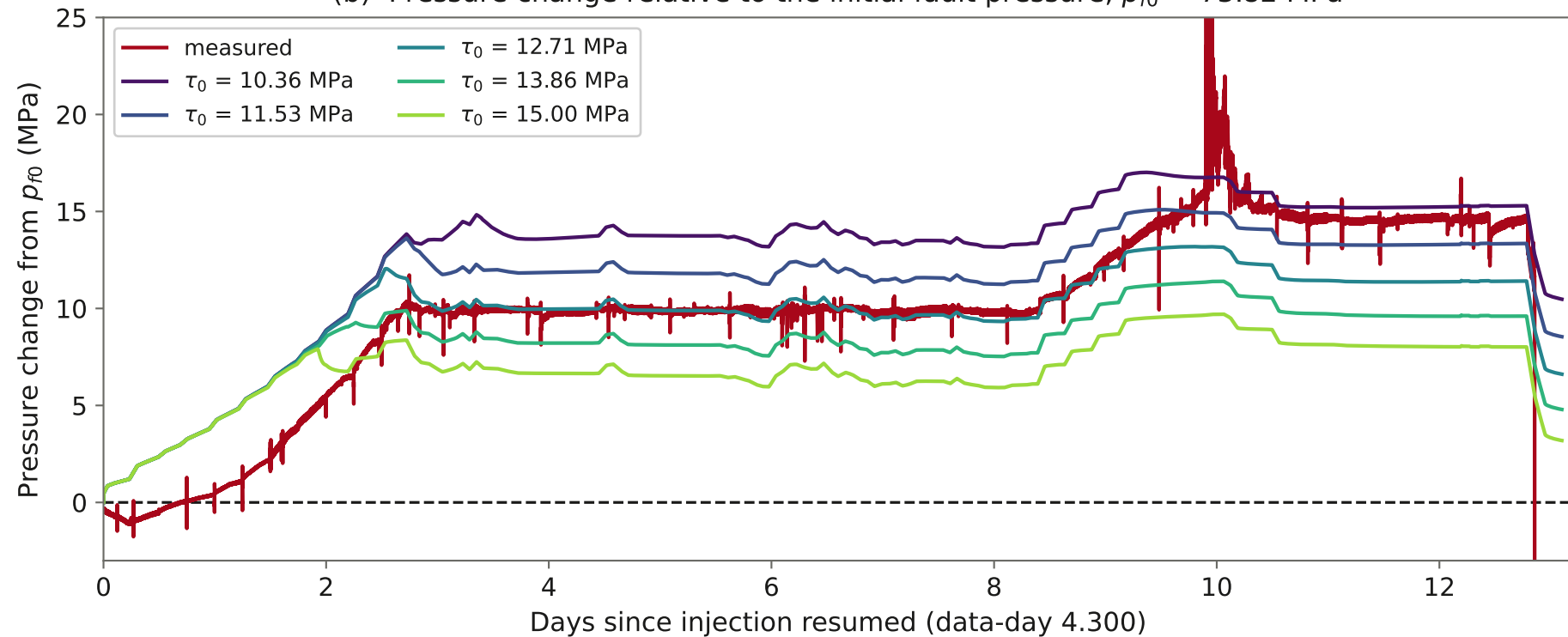
(b) Pressure change relative to the initial fault pressure, p_{f0} = 73.82 MPa
