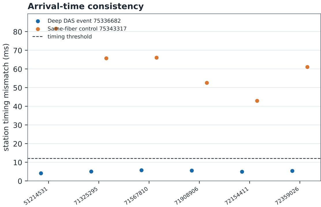
A and B show the same DAS processing for a deep event and a same-fiber control. C and D compare each event with six known family earthquakes using the frozen seismic-network test. The family label remains provisional because published catalogs disagree.
