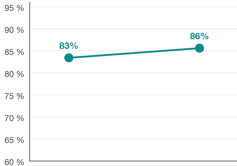
Algorithm GLM 5.2 → 5.3
