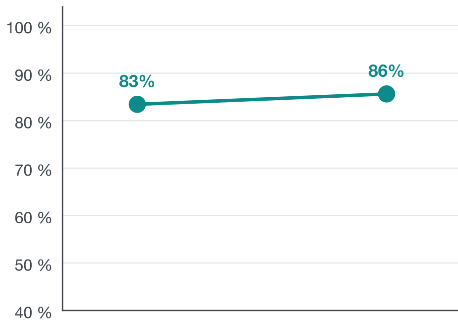
Algorithm GLM 5.2 → 5.3
