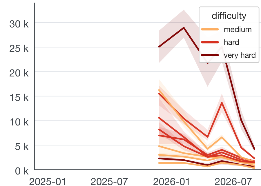
Mean output tokens (correct traces)
