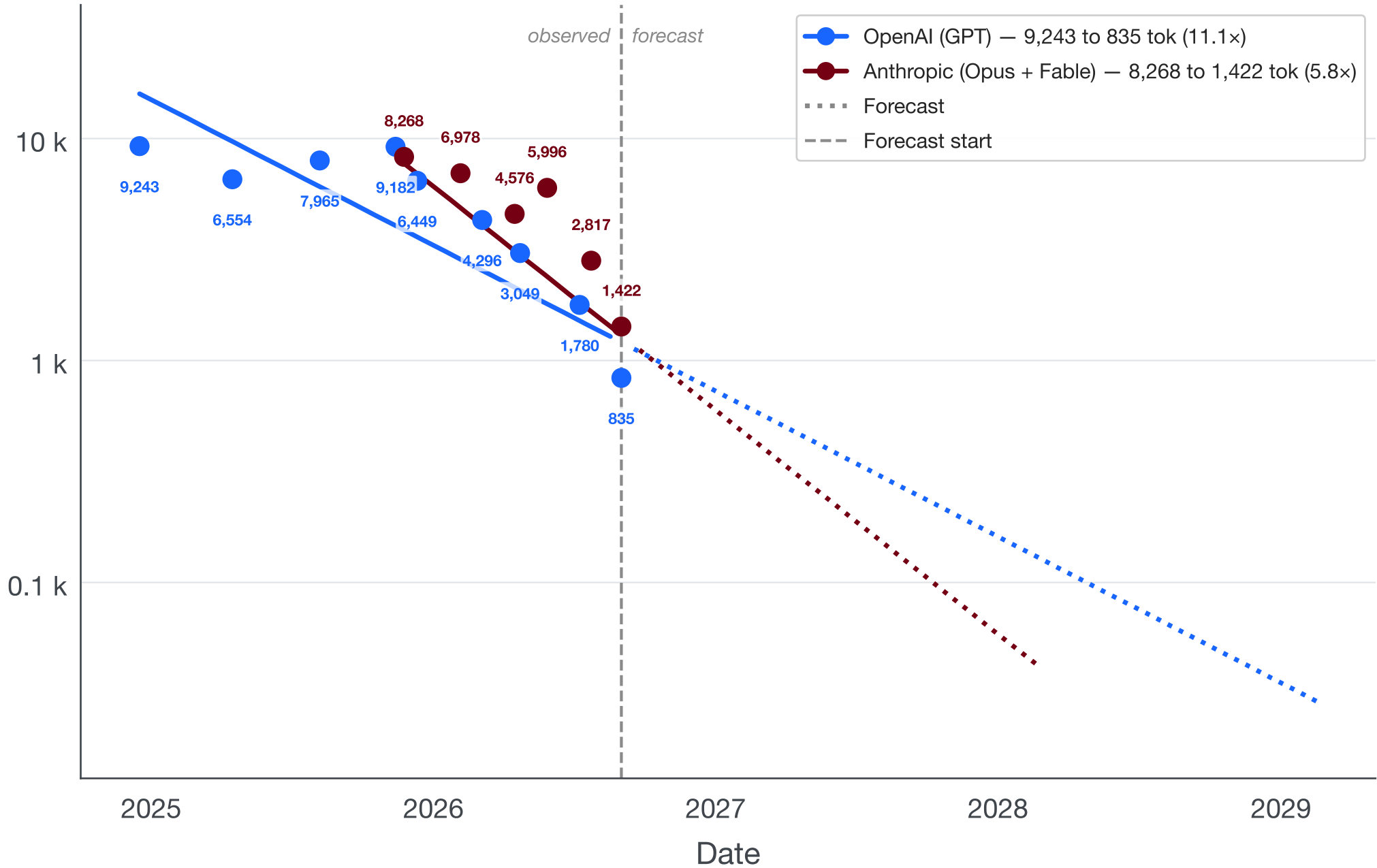
Mean excess over the floor (output tokens)
