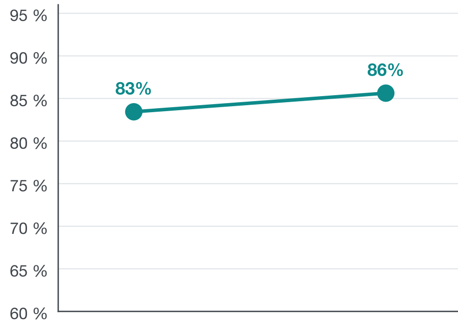
Algorithm GLM 5.2 → 5.3
