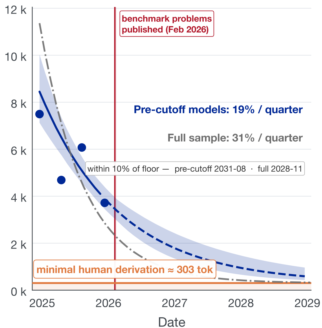
OpenAI (GPT) — pre-cutoff models only
