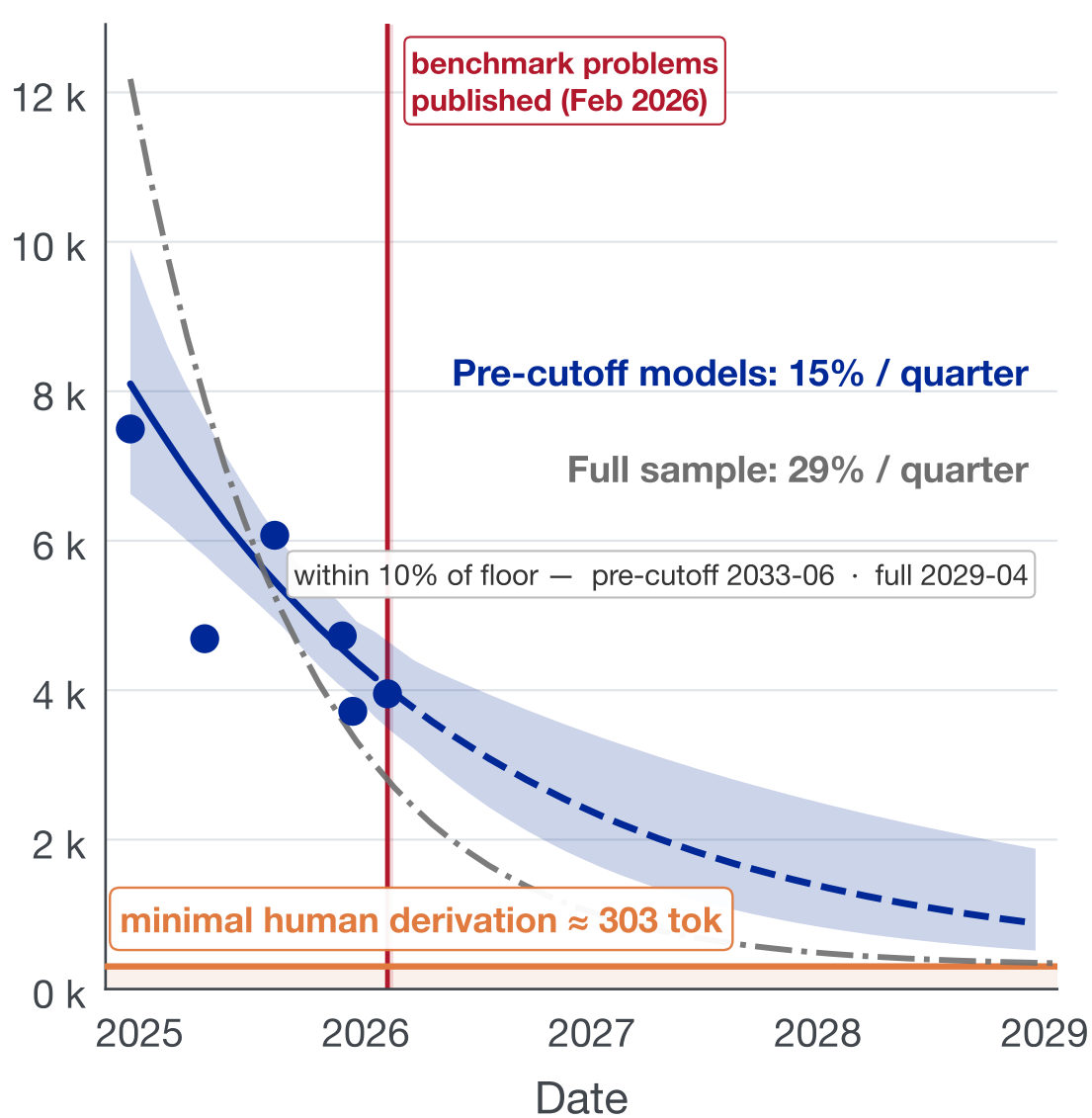
GPT + Opus pooled — pre-cutoff models only
