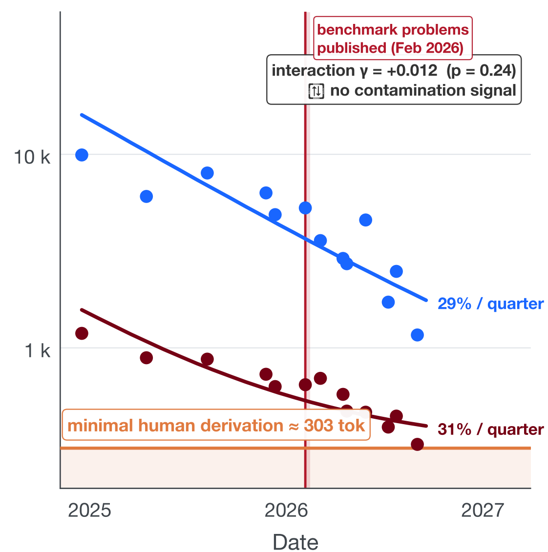
Same models, problems split by vintage (full window — breaks the tie)
