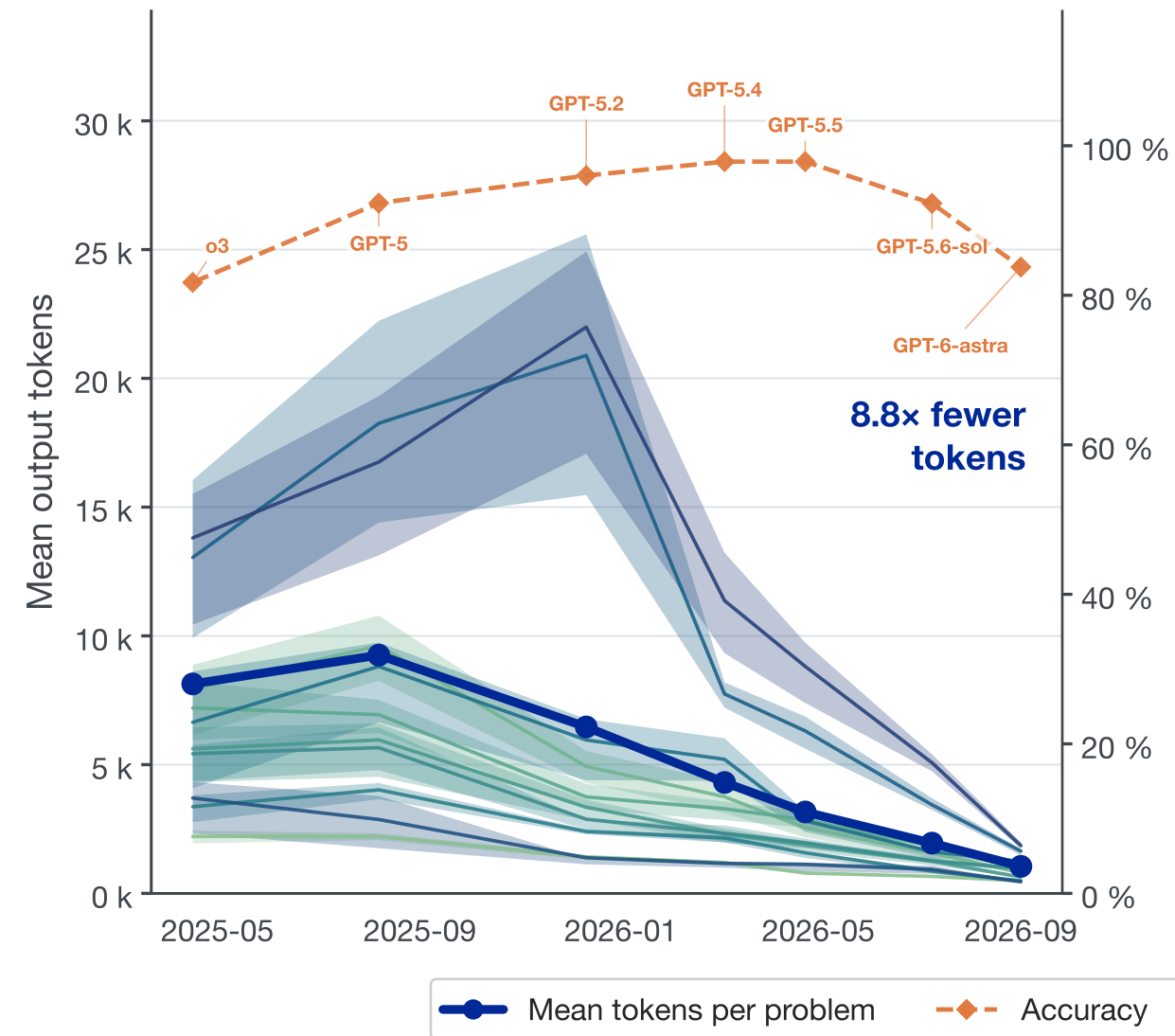
OpenAI (GPT)
