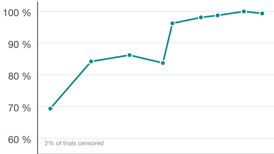
OpenAI (GPT)
