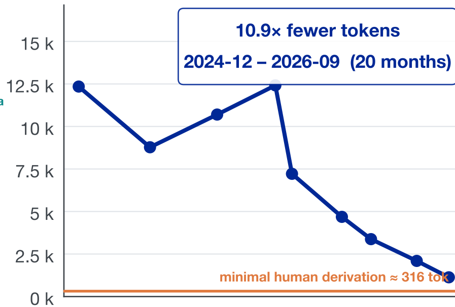
Mean output tokens (all attempts)
