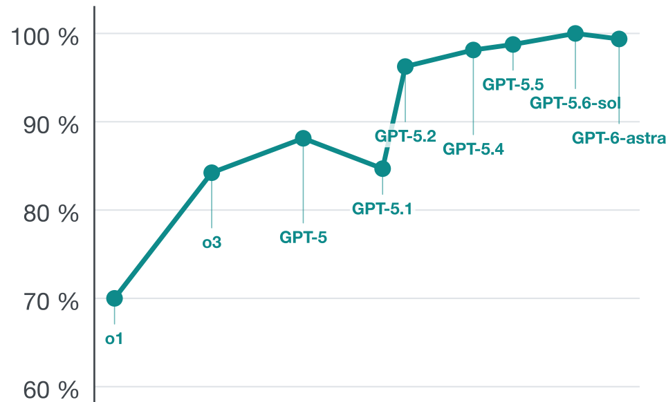
Accuracy
