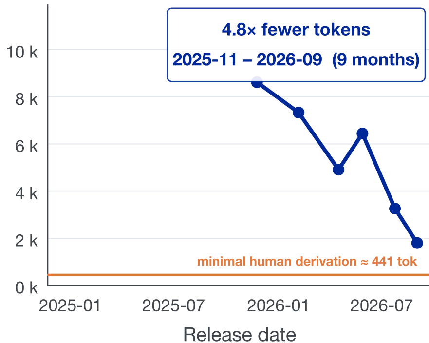
Output tokens by problem (hard-but-doable, correct traces)
