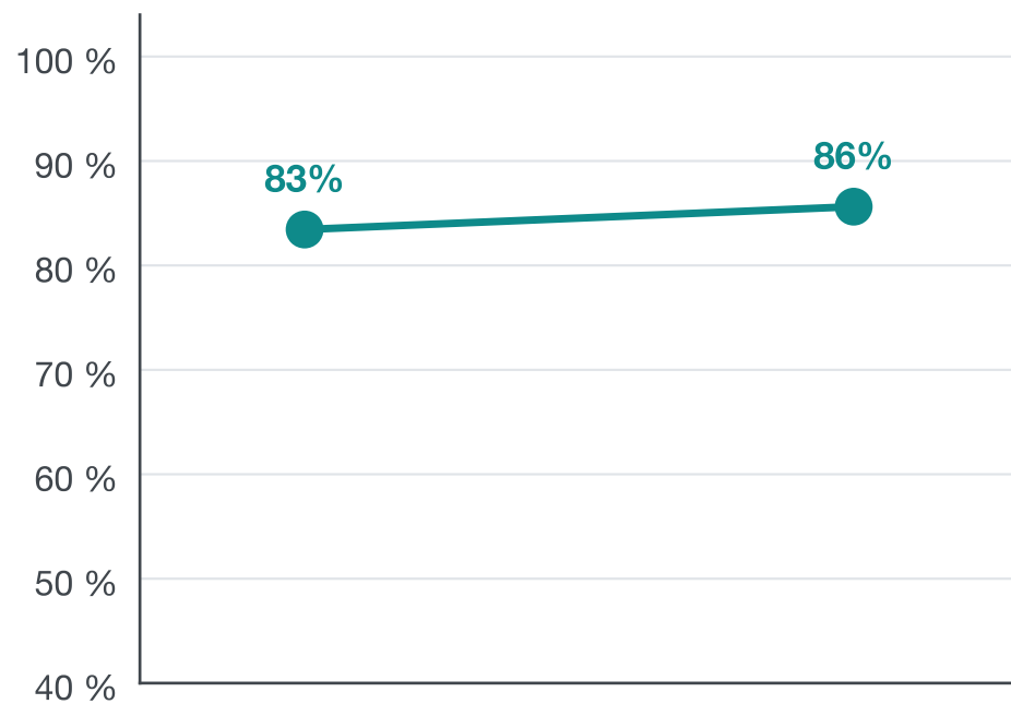
Algorithm GLM 5.2 → 5.3
