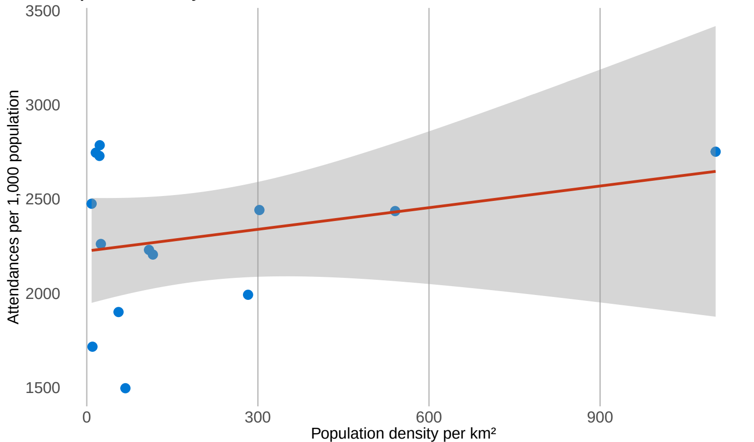
Population density and A&E attendance rates
