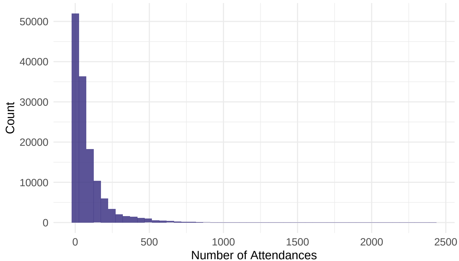
Distribution of NumberOfAttendances (per row)
