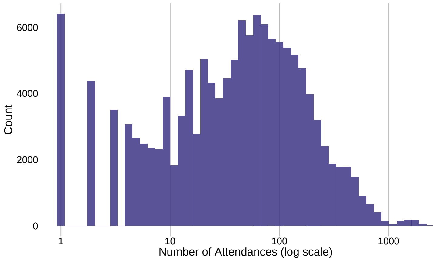
Distribution of Number Of Attendances (log scale)
