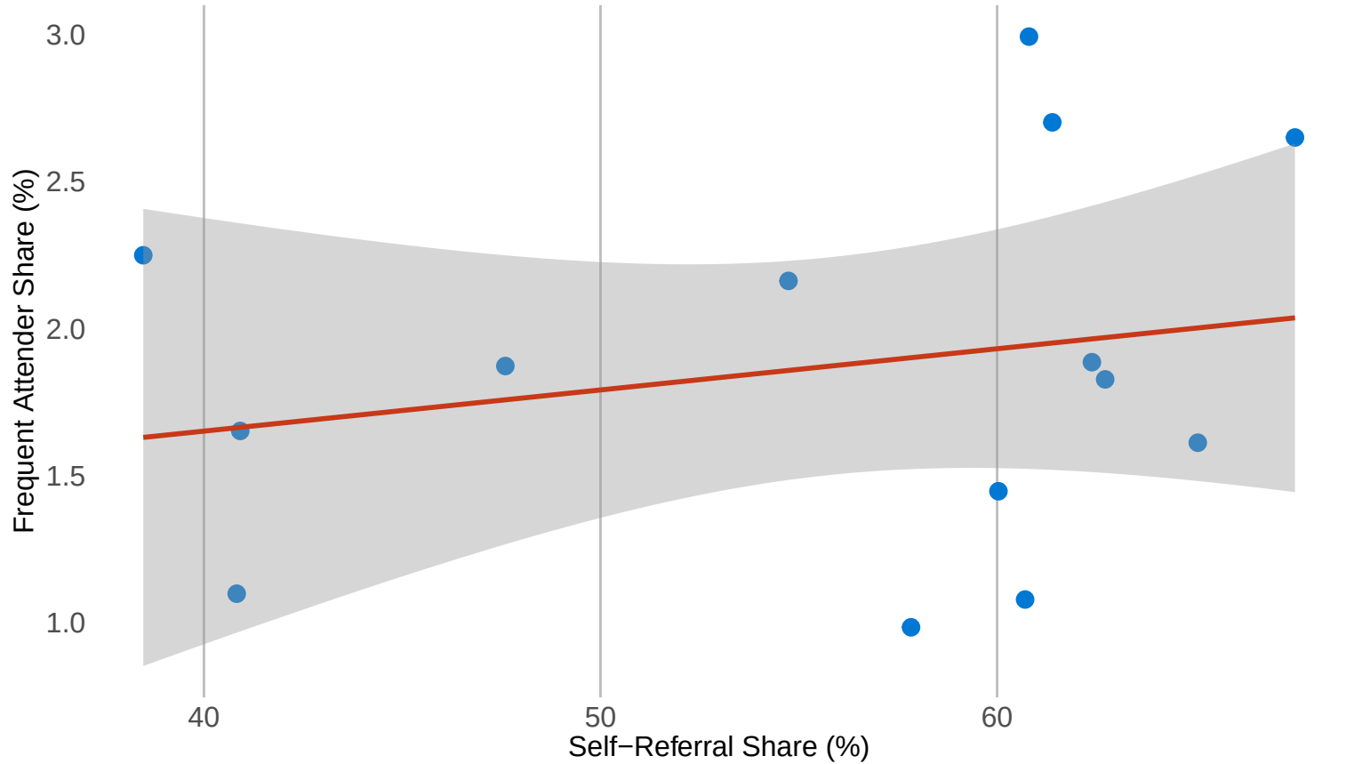
Self-Referral Rate vs. Frequent Attendance Rate, by Health Board
