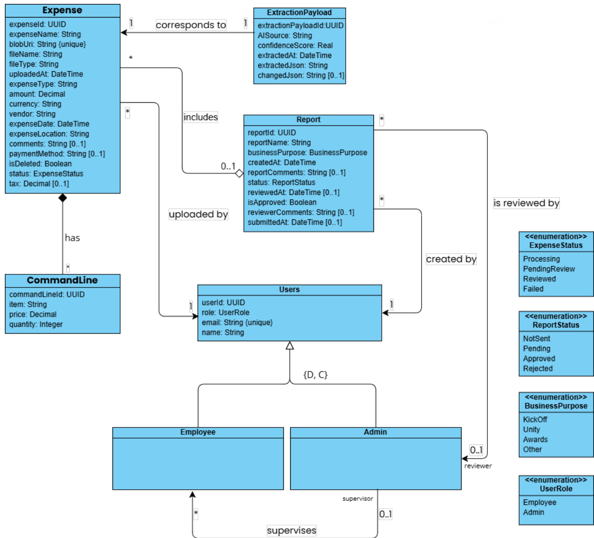
Figure 7.2.1: Conceptual data schema. [Own creation]
