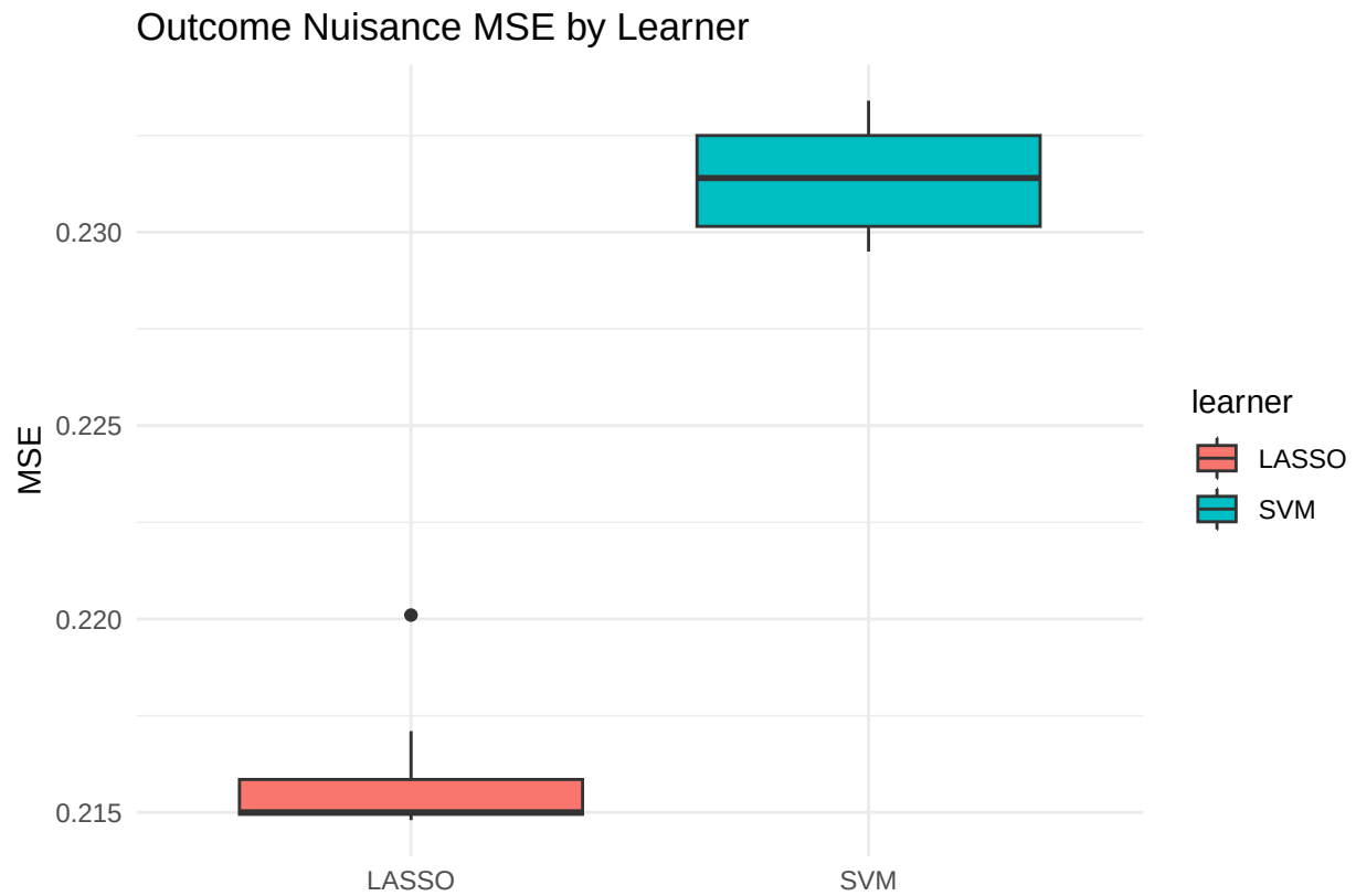
Figure 3: Model Comparison
