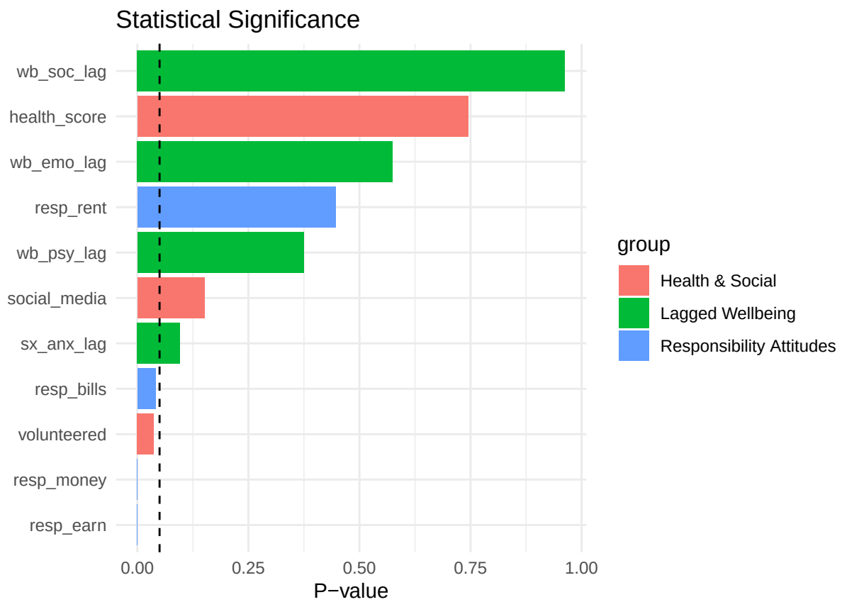
Figure 2: P-values
