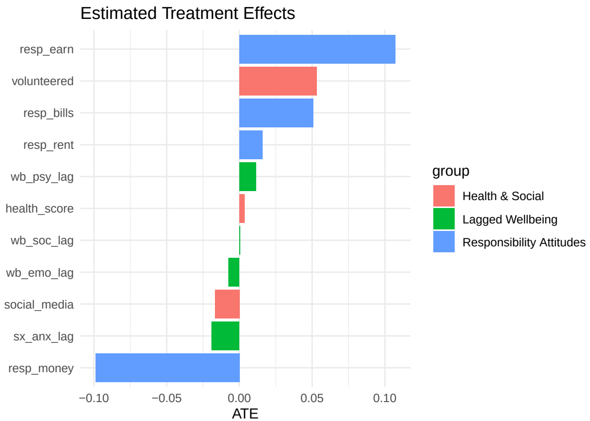
Figure 1: ATE Estimates
