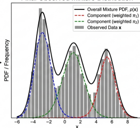
Final Observed Mixture Distribution
