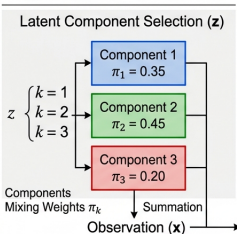
Component Distributions ( k=1, 2, 3 )
