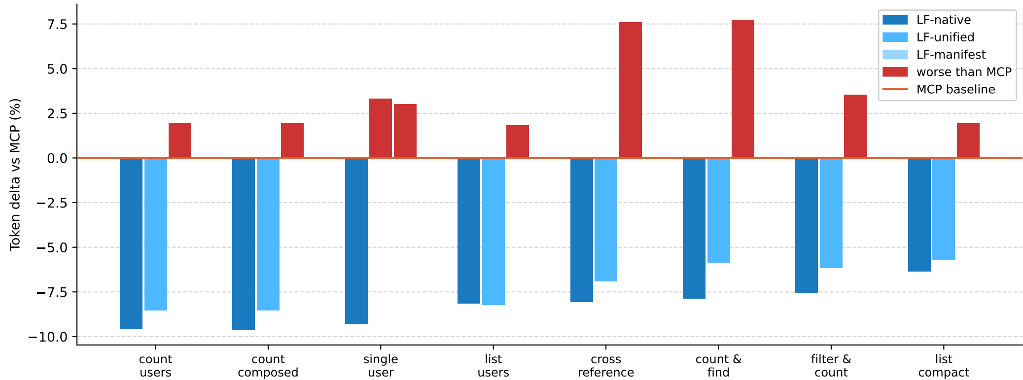
Token efficiency relative to MCP (negative = fewer tokens than MCP)
