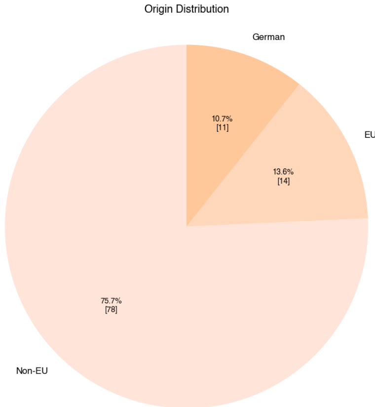
Figure 44. Origin Distribution
