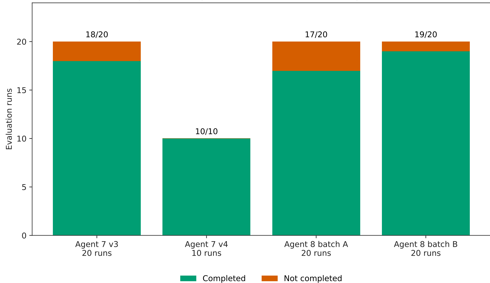
Figure 10.5: Repeated-evaluation outcome composition
