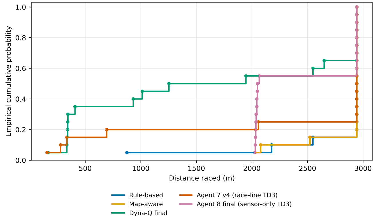
Distribution of progress across all valid attempts
