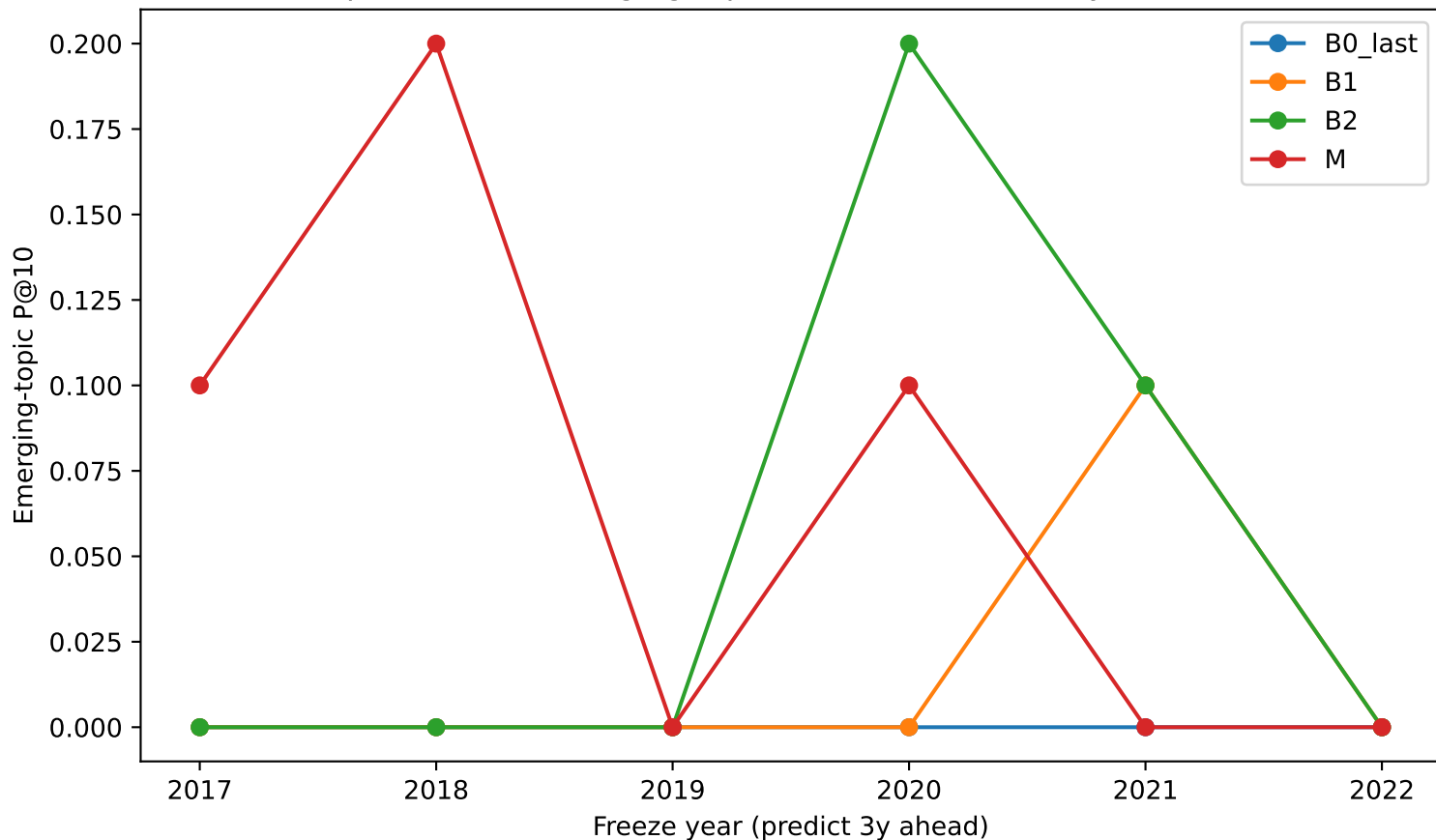
Experiment 2: emerging topic hit rate over freeze years (h=3)
