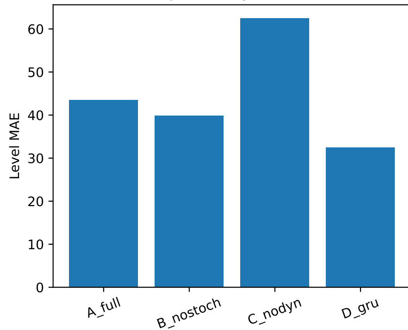
Horizon 5y (val targets 2016-2020)
