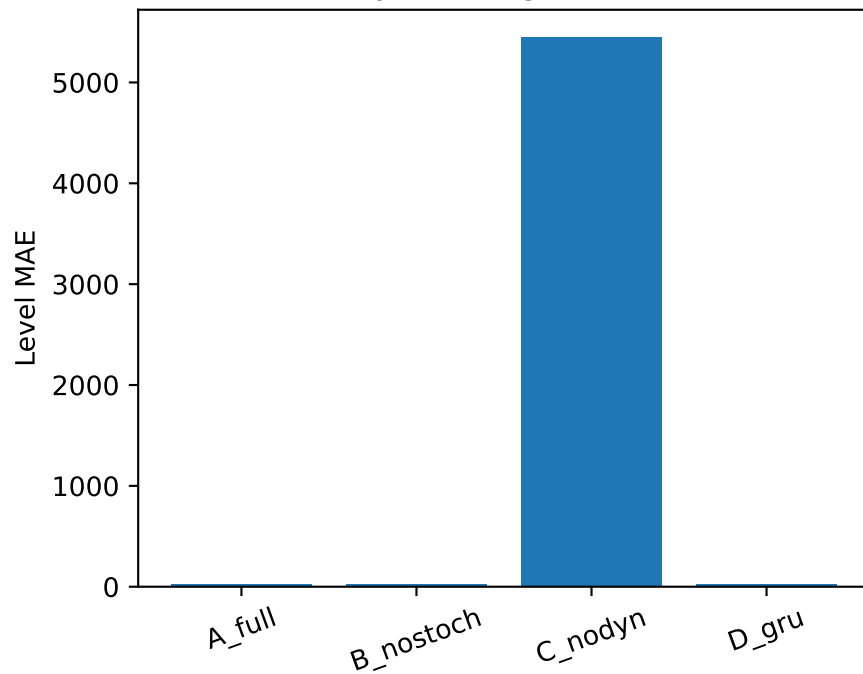
Horizon 3y (val targets 2016-2020)
