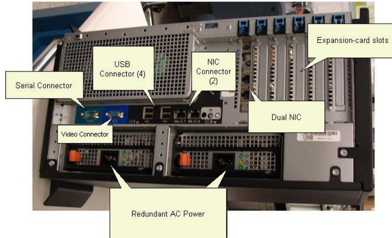
Figure 2-1 PE2900-based Back Panel Connections
