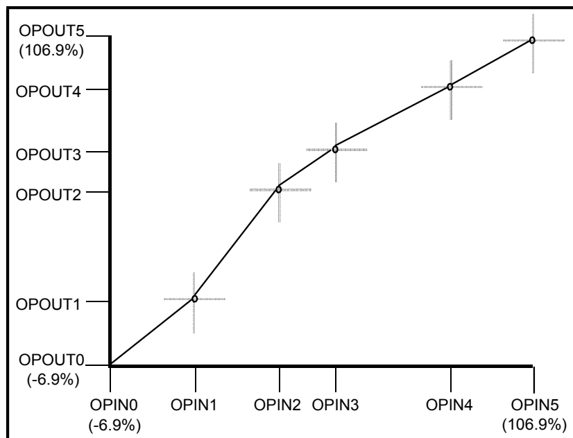
Figure 2-6 — Output Characterization for Analog Output Point
