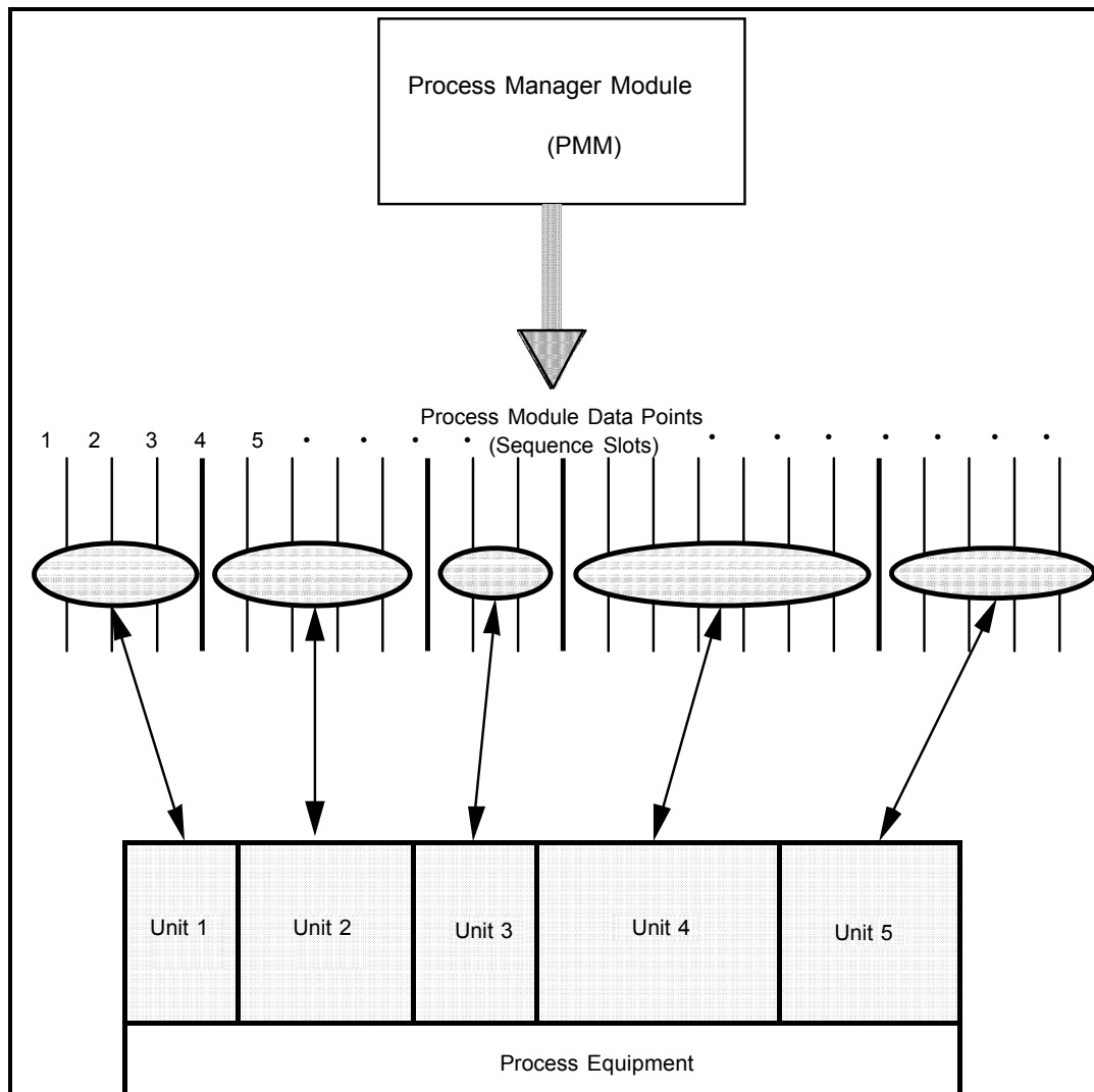
Figure 6-2 — Sequence Program Partitioning/Unit Partitioning
