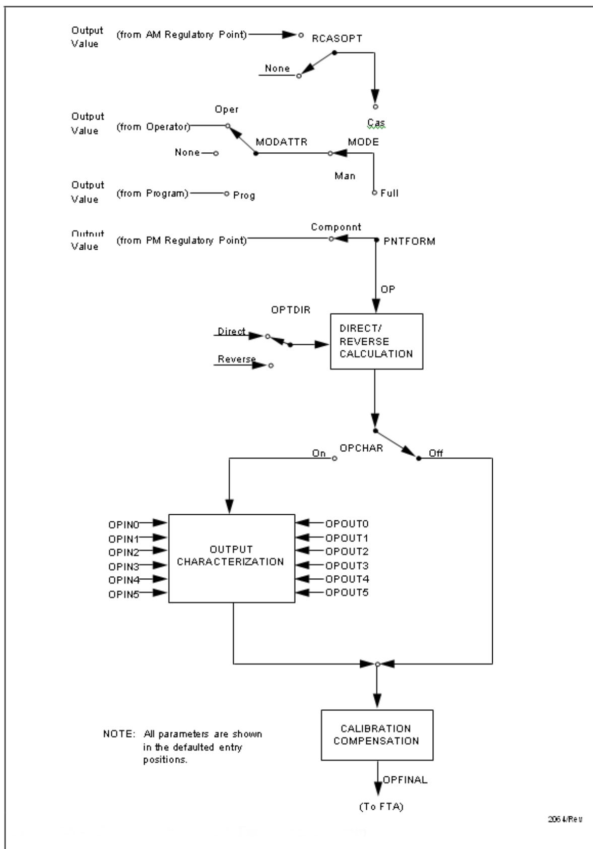
Figure 2-5 — Analog Output Point, Functional Diagram
