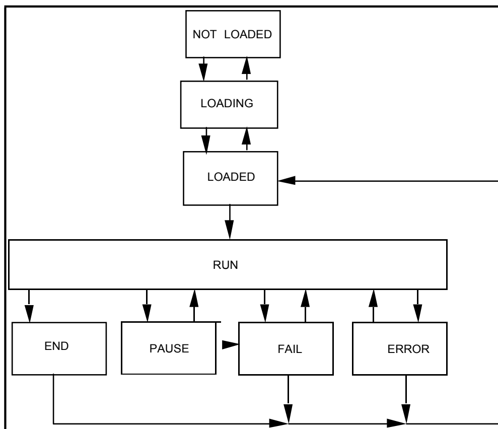
Figure 6-6 — Sequence Execution States
