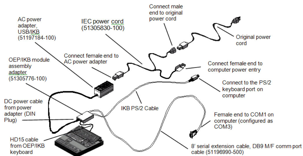
Figure 2-8 OEP/IKB Adapter Connections for IKB
