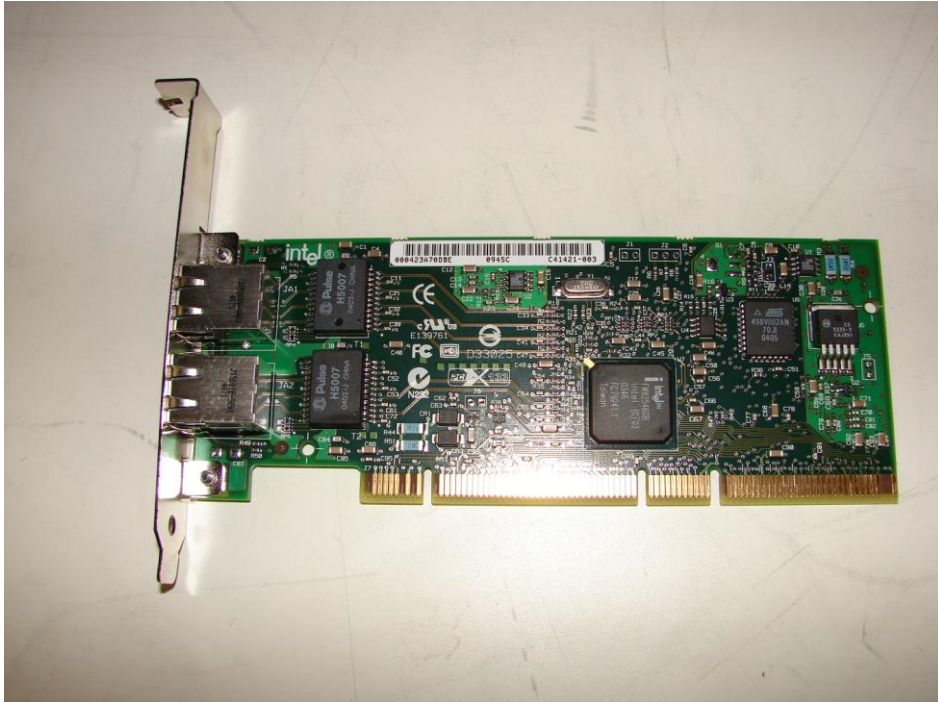
Figure 4-1 LCNP4M Board
