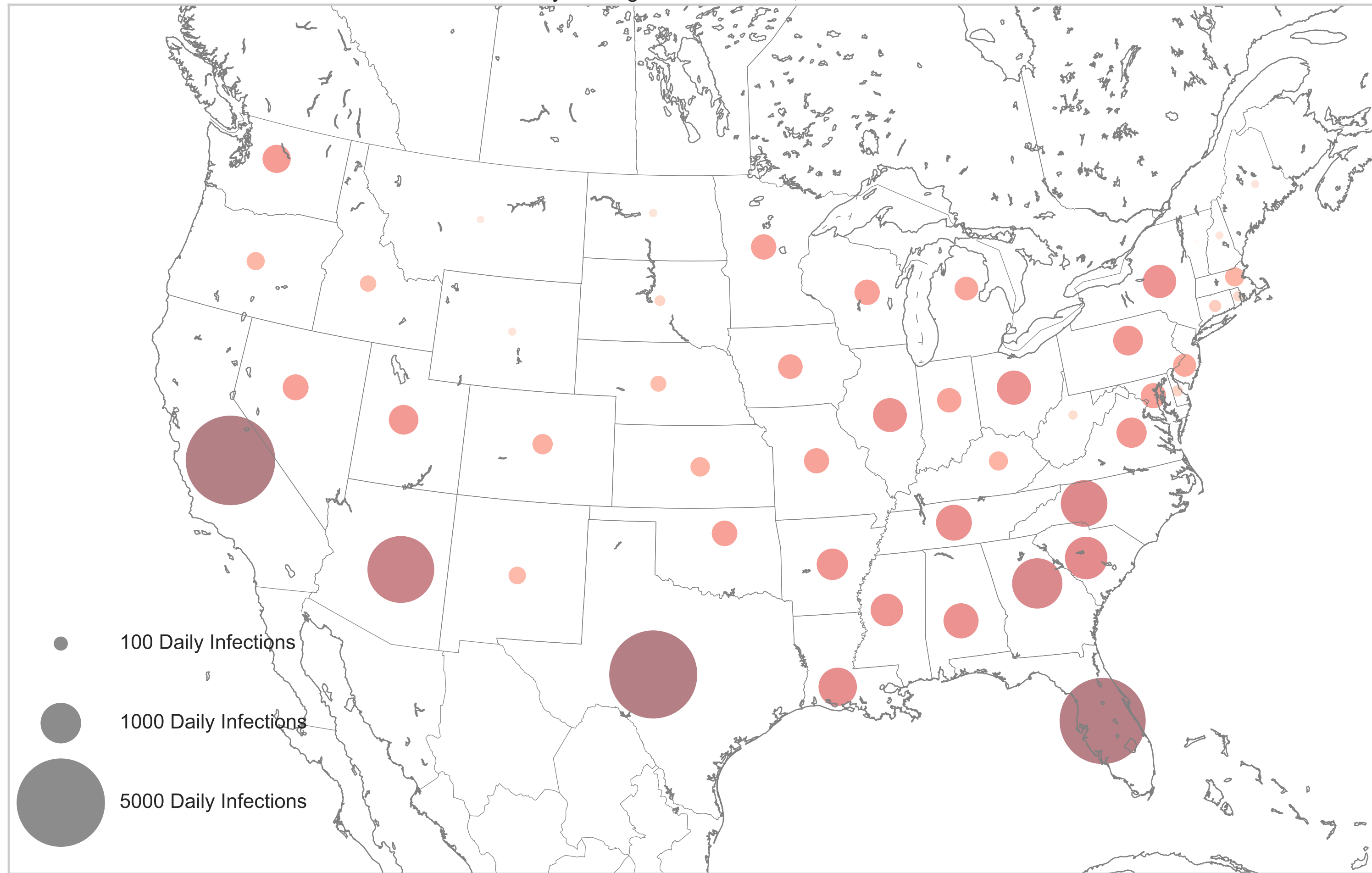
7 Day Average Infection Rate, 6/26/20
