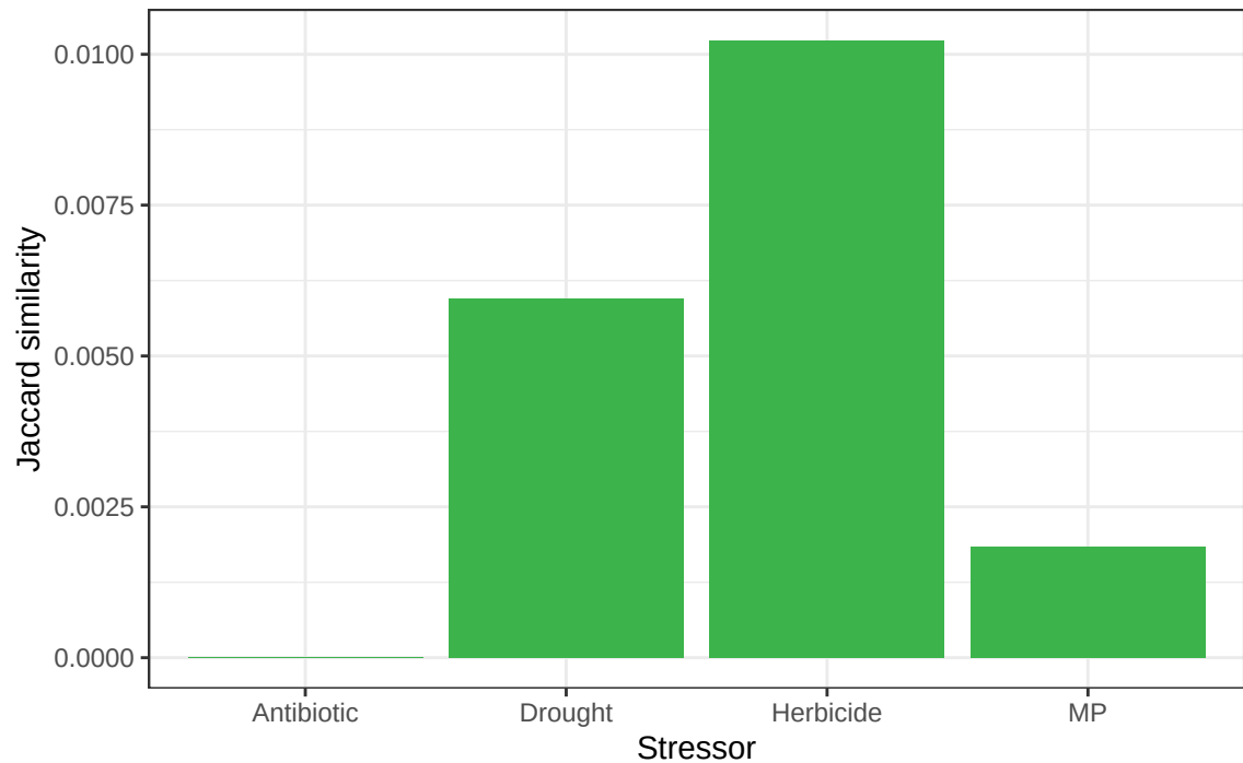
Edge overlap: present vs. absent networks
