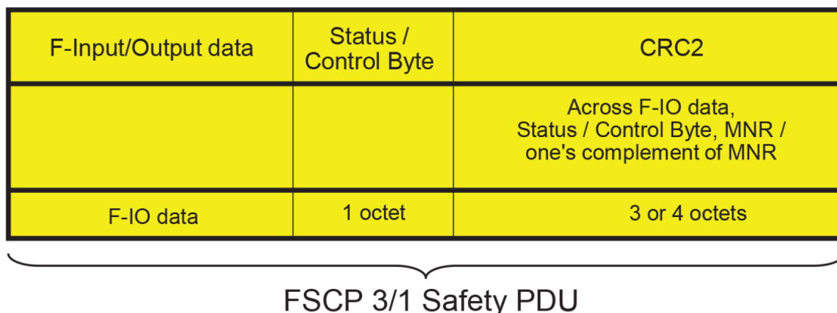
Figure 2.3: PROFIsafe frame format
