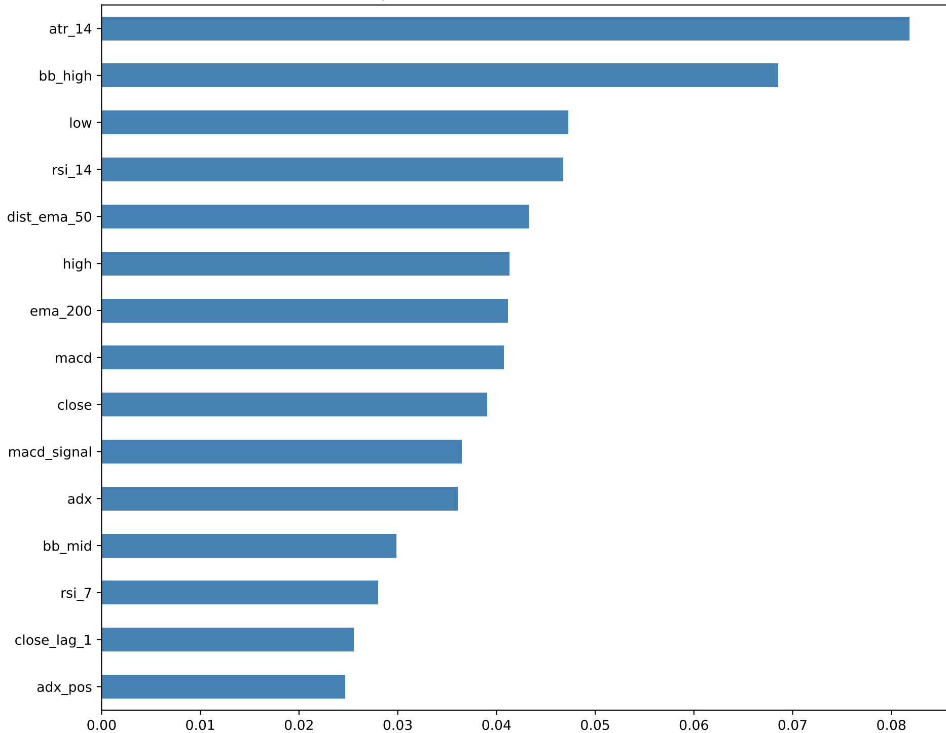
Top 15 Features - Bear Trend (Classifier)
