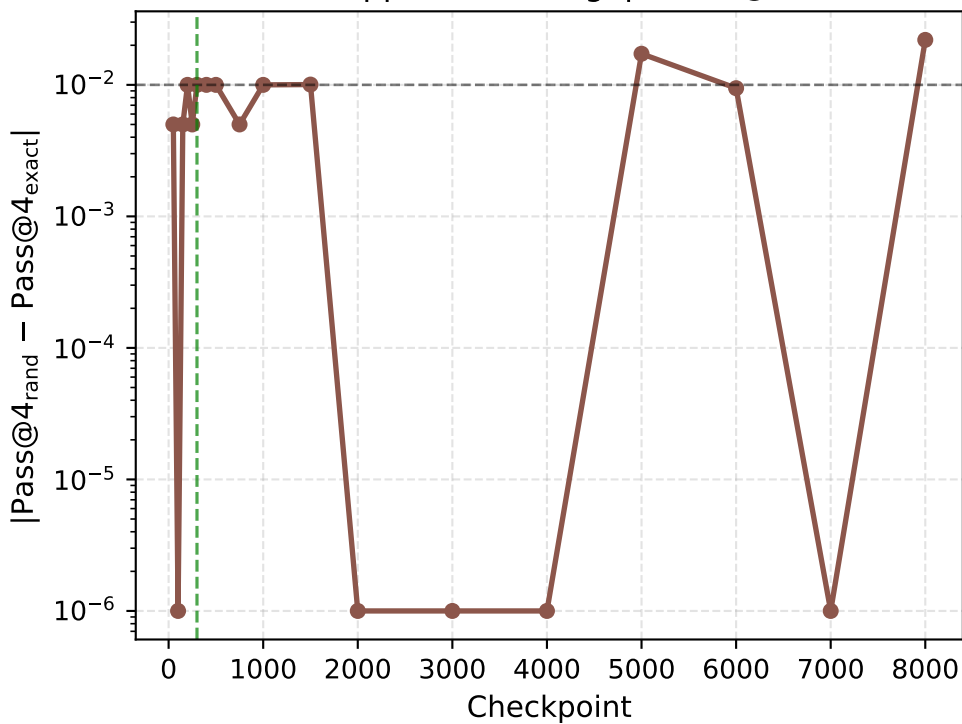
D. Approximation gap (Pass@4)
