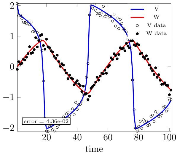
Inexact prox ( \kappa_s = 10^{-7} )
