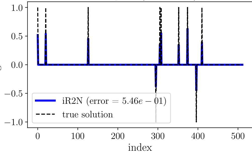
Exact prox ( \kappa_s = 10^{-7} )
