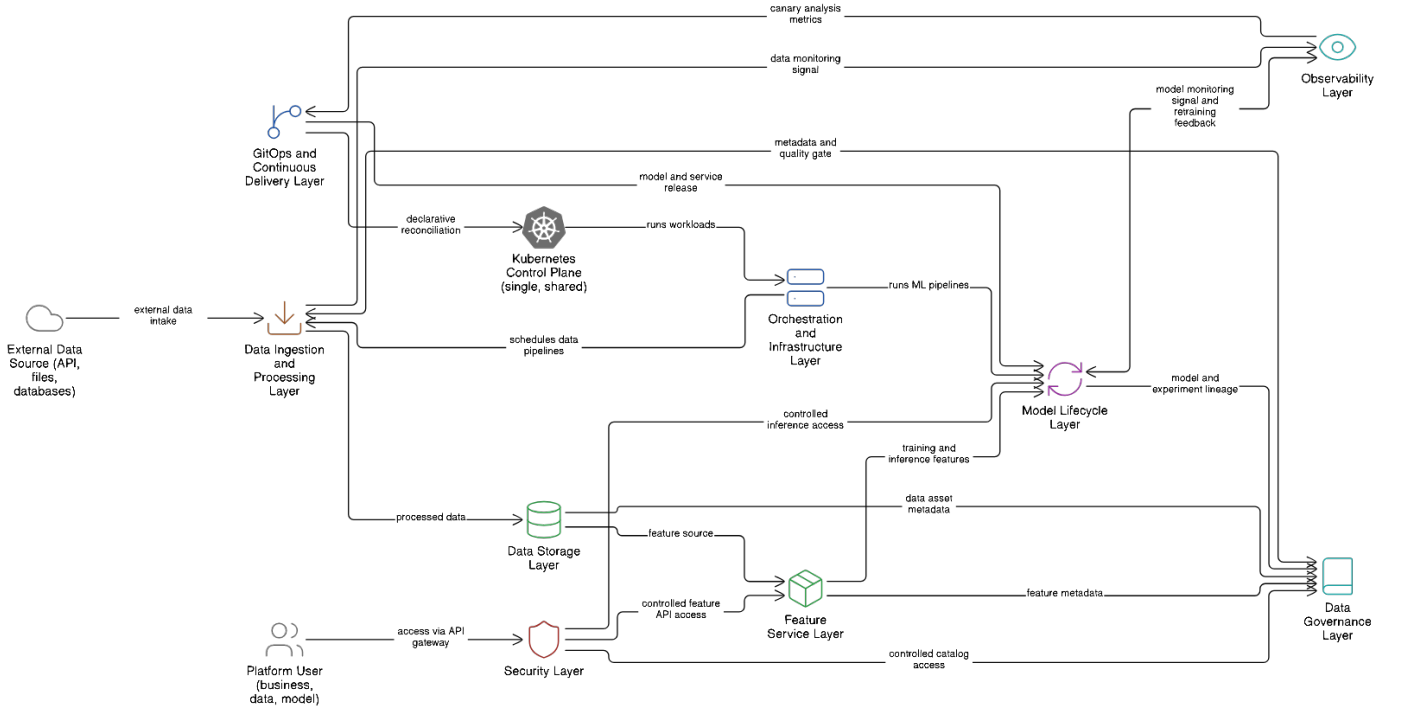
Fig. 1. Integrated service architecture across the nine layers on one Kubernetes control plane, drawn without binding to any tool [12]
