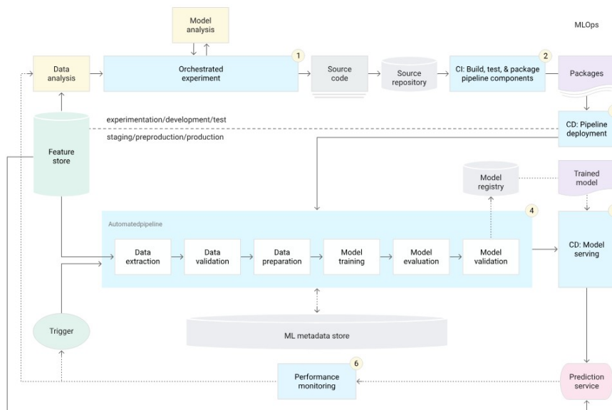
Gambar II.5 MLOps level 2 : orkestrasi CI/CD/CT (Google Cloud 2024)
