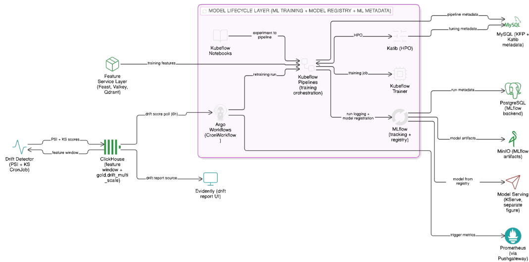
Gambar IV.6 Rincian Model Lifecycle Layer
