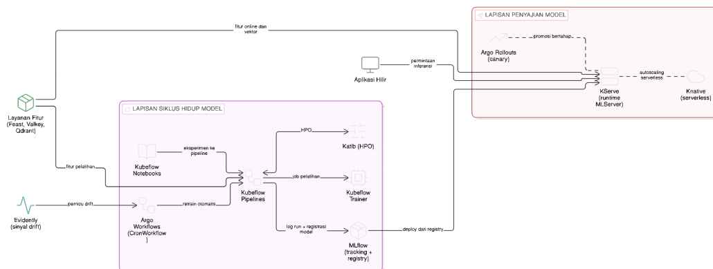
Gambar IV.16 Rincian Model Lifecycle Layer
