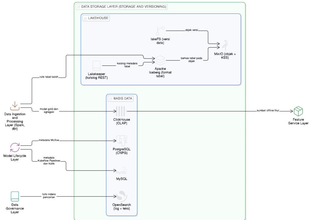
Gambar IV.4 Rincian Data Storage Layer
