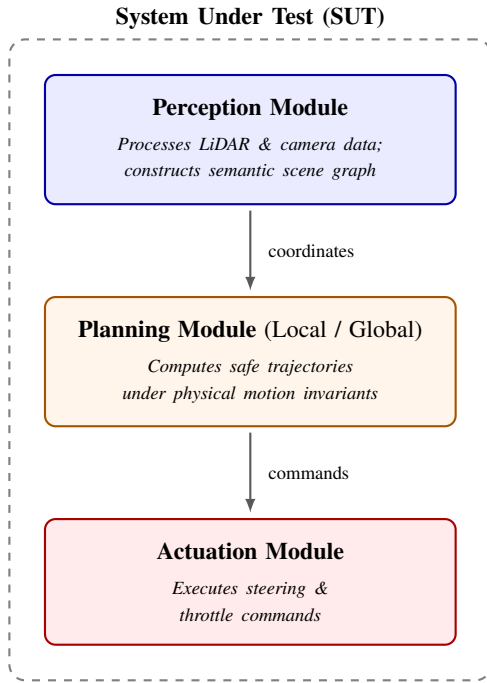
Fig. 8. Reference architecture for an autonomous CPS System-Under-Test. The three modules—Perception, Planning, and Actuation—correspond to distinct abstraction tiers whose interfaces are modelled as states and transitions in the NeSy-MBST usage model.
