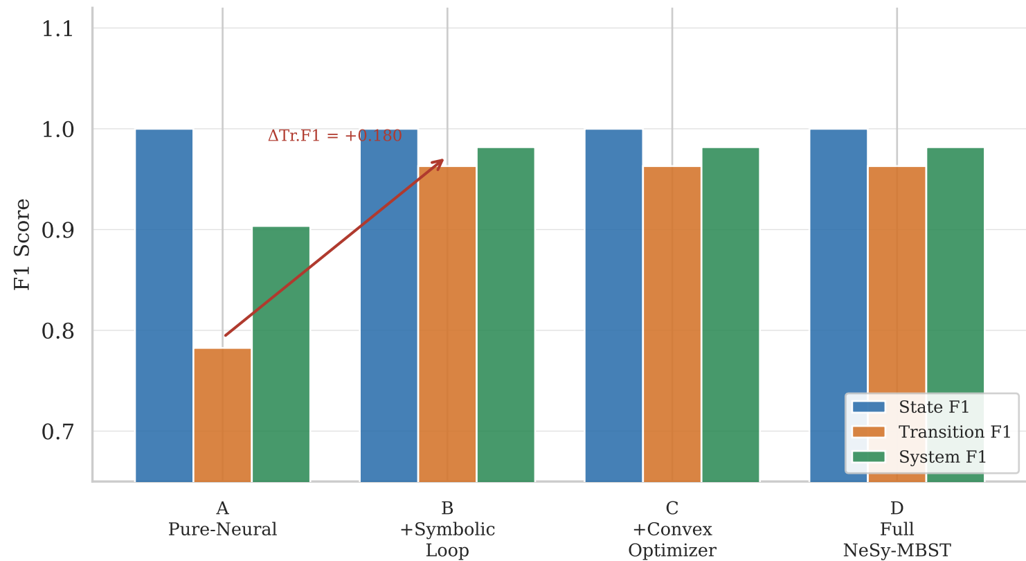
Ablation Study: F1 Scores on AV CPS Benchmark (Each condition adds one NeSy-MBST component)
