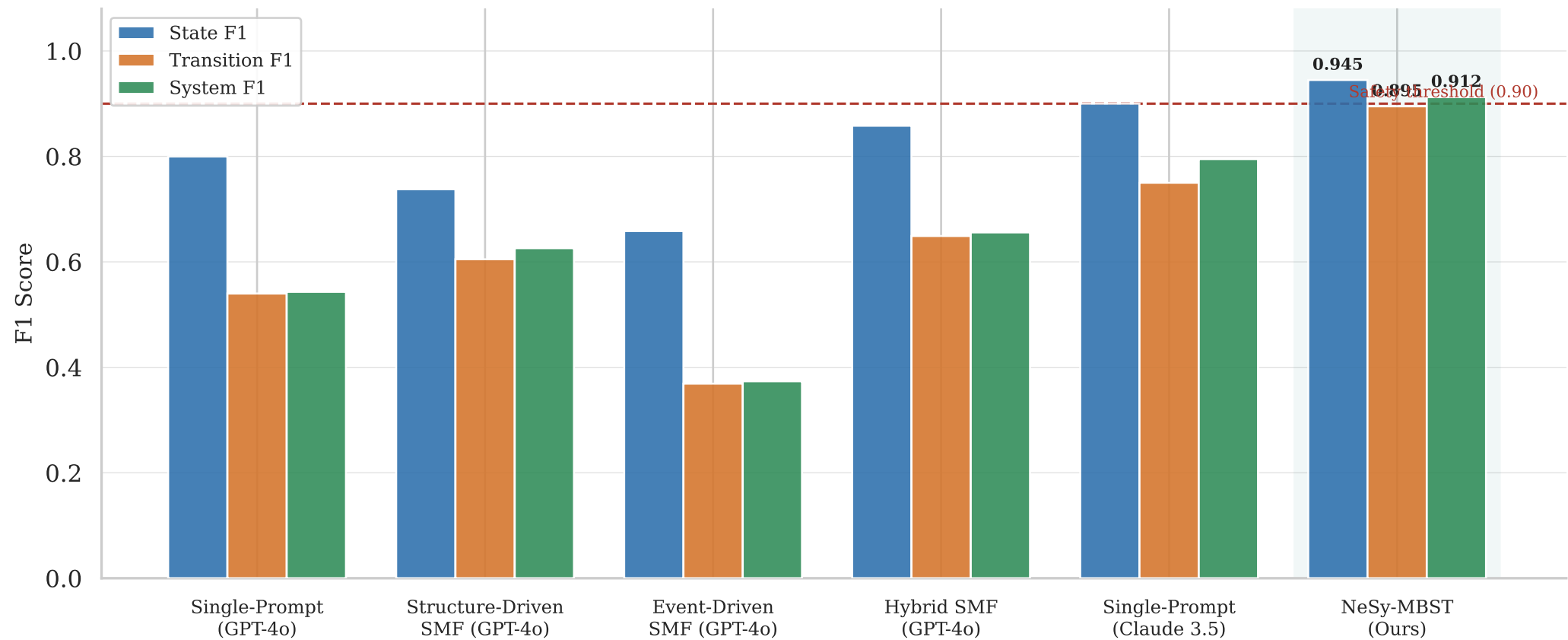
State, Transition, and System F1 Scores Across Prompting Strategies
