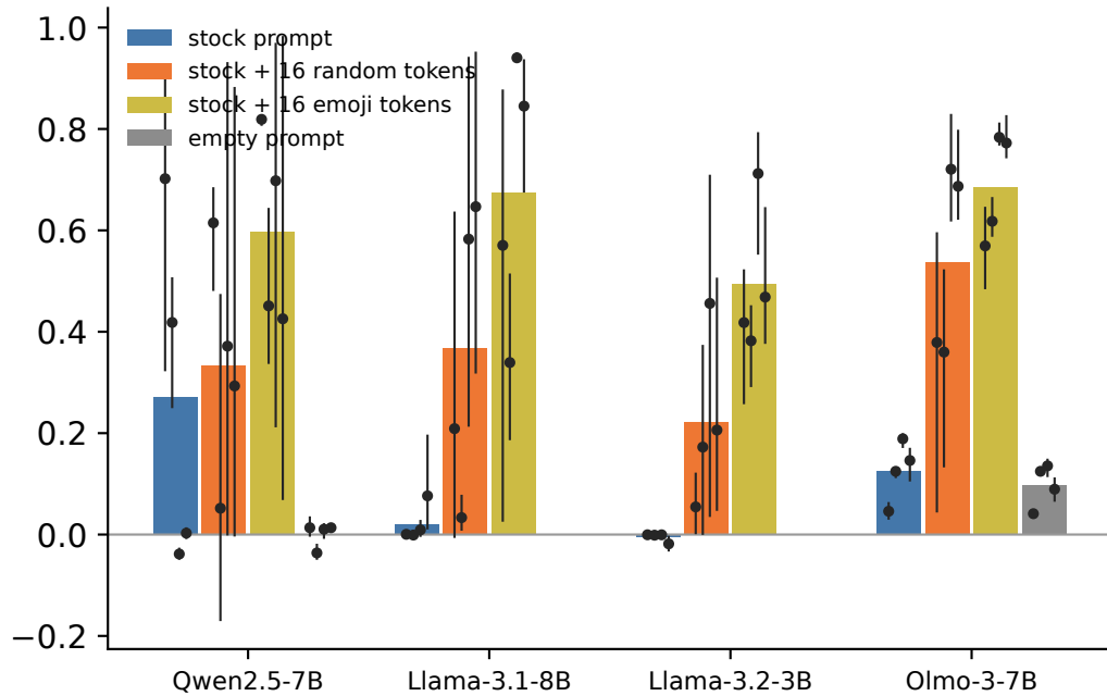
fixed lr (3e-4), 3 seeds per animal dot = animal's seed mean, line = its seed range
