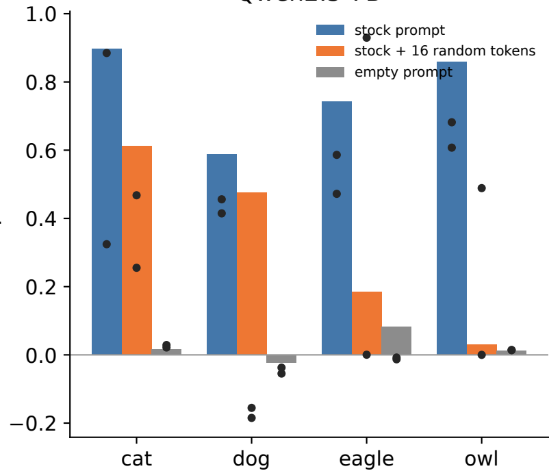
Qwen2.5-7B
