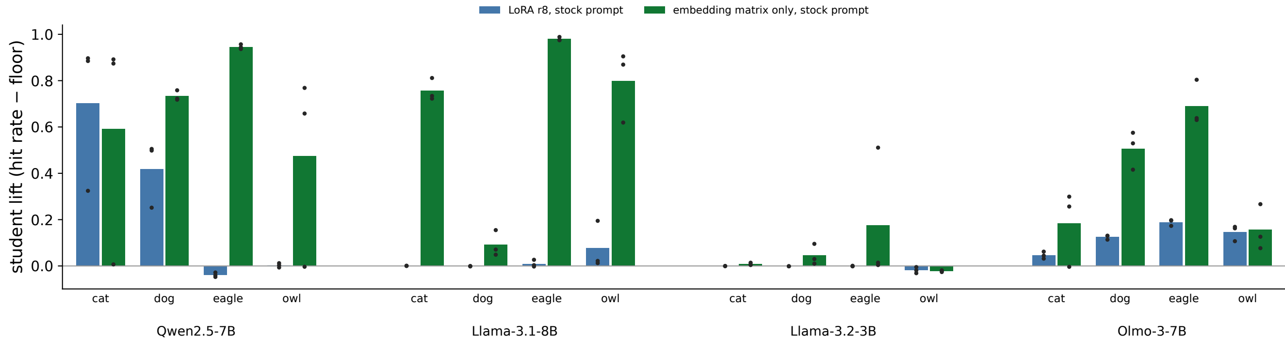
fixed lr (LoRA 3e-4, embed 1e-3): bar = mean over seeds, dots = seeds
