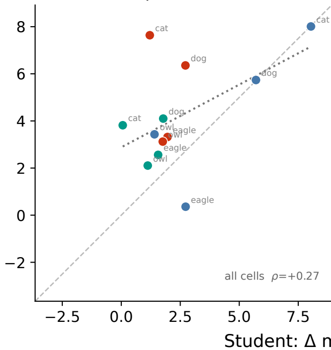
Prompted teachers
