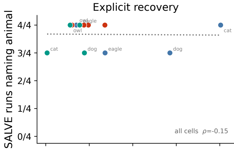
Prompted teachers
