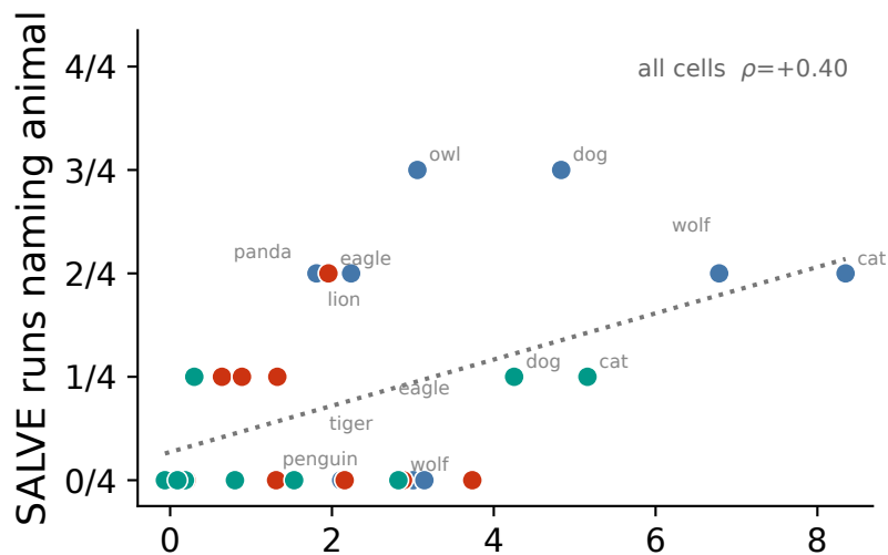
Steered teachers
