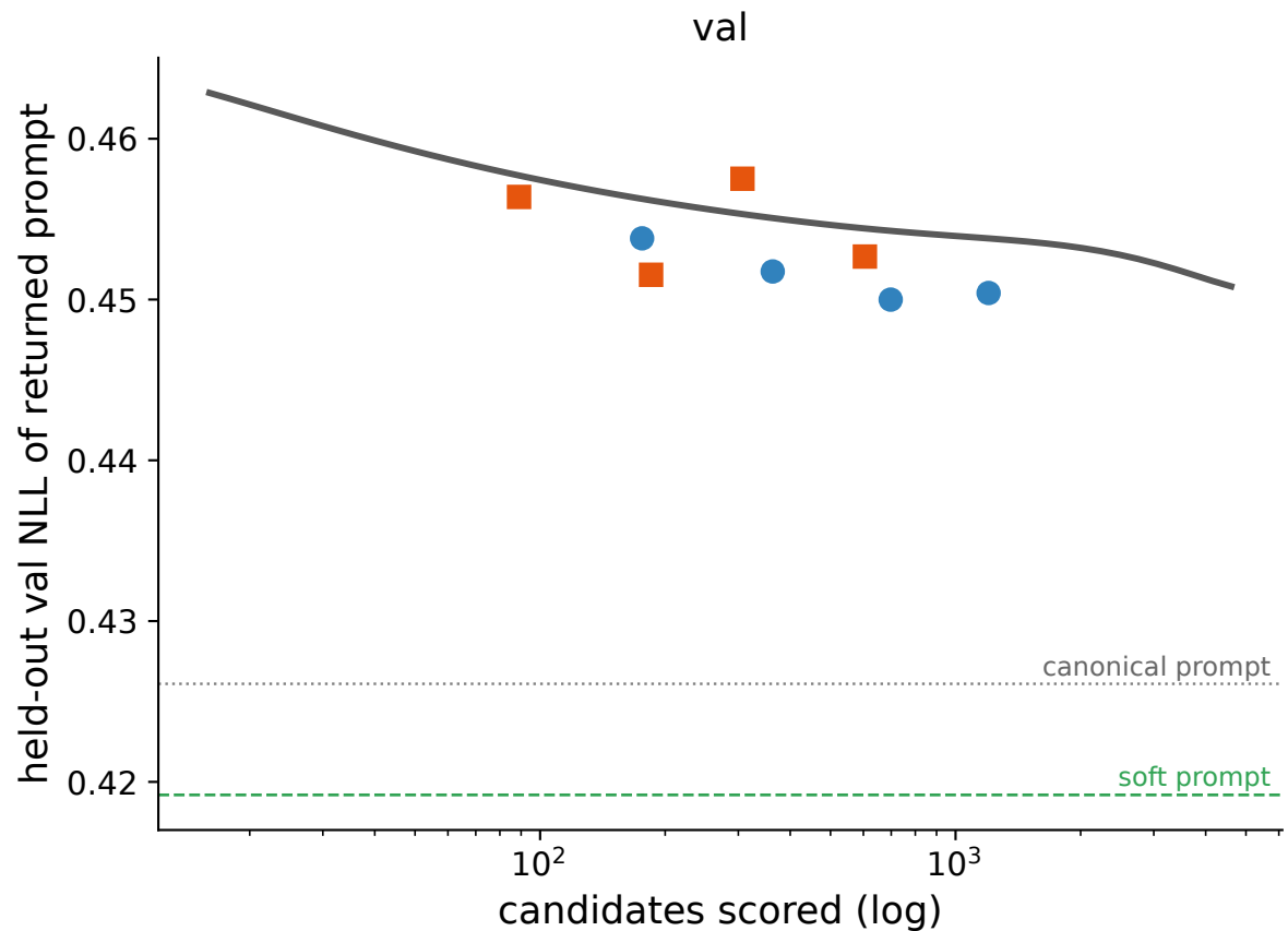
beam vs best-of-N (cat, seed 42)
