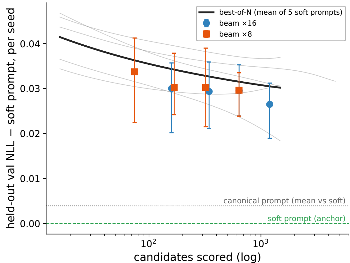
val — beam vs best-of-N (cat, all 5 soft prompts)
